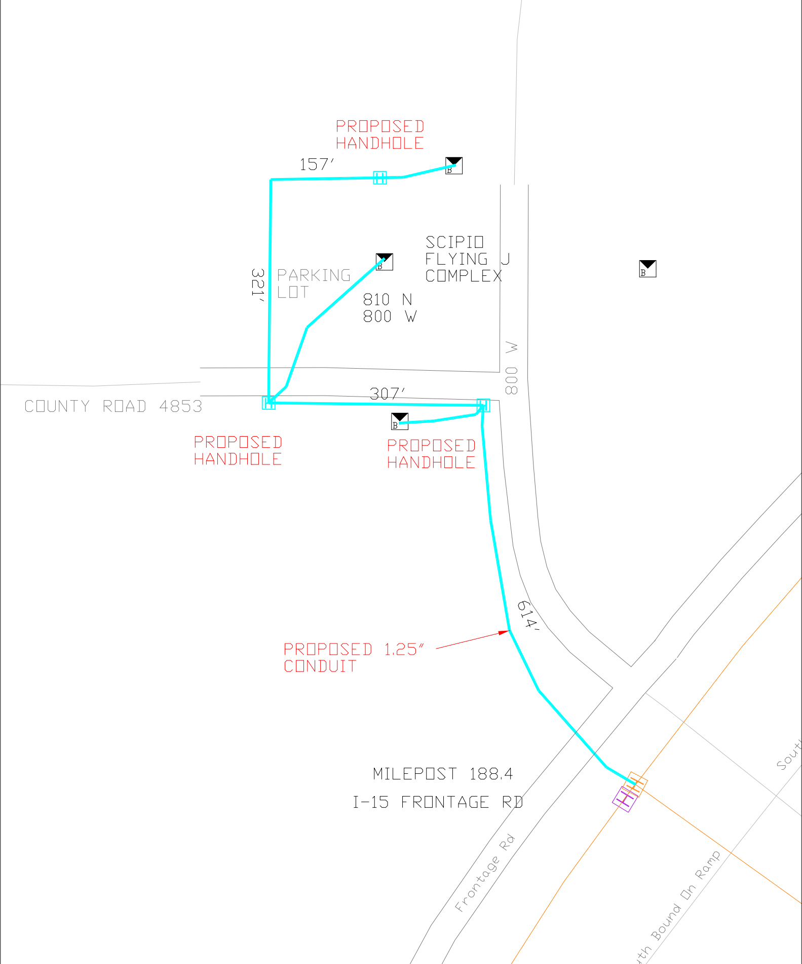
CentraCom, MC198182: Proposed conduit path to Scipio Flying J Complex, 810 N 800 West, Scipio, UT. Accessing existing handhole at Milepost 188.4 between I-15 Southbound on-ramp and Frontage Road, Millard County, UT.
