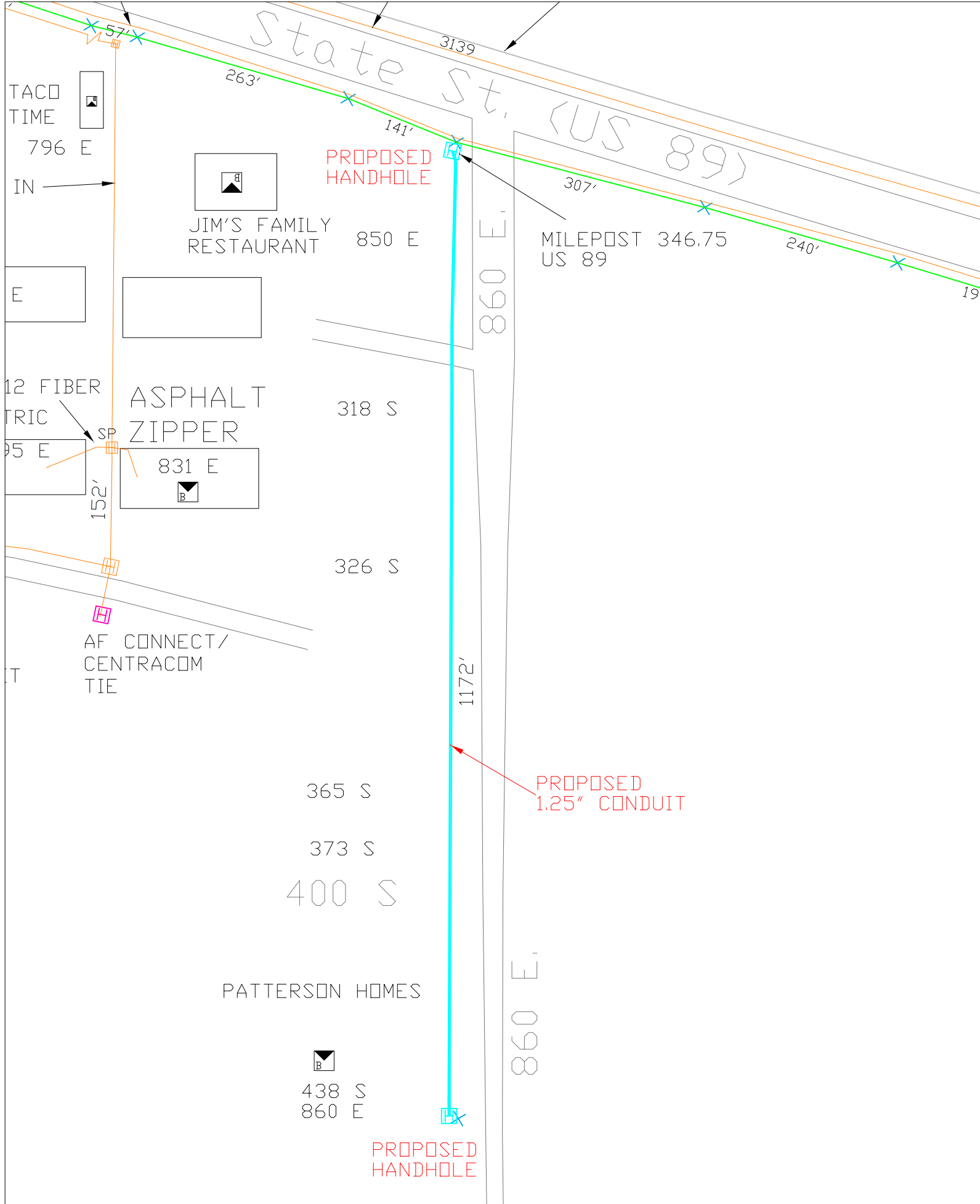
CentraCom, MC198044: Proposed conduit path to Patterson Homes, 438 S 860 East, American Fork City, UT.
