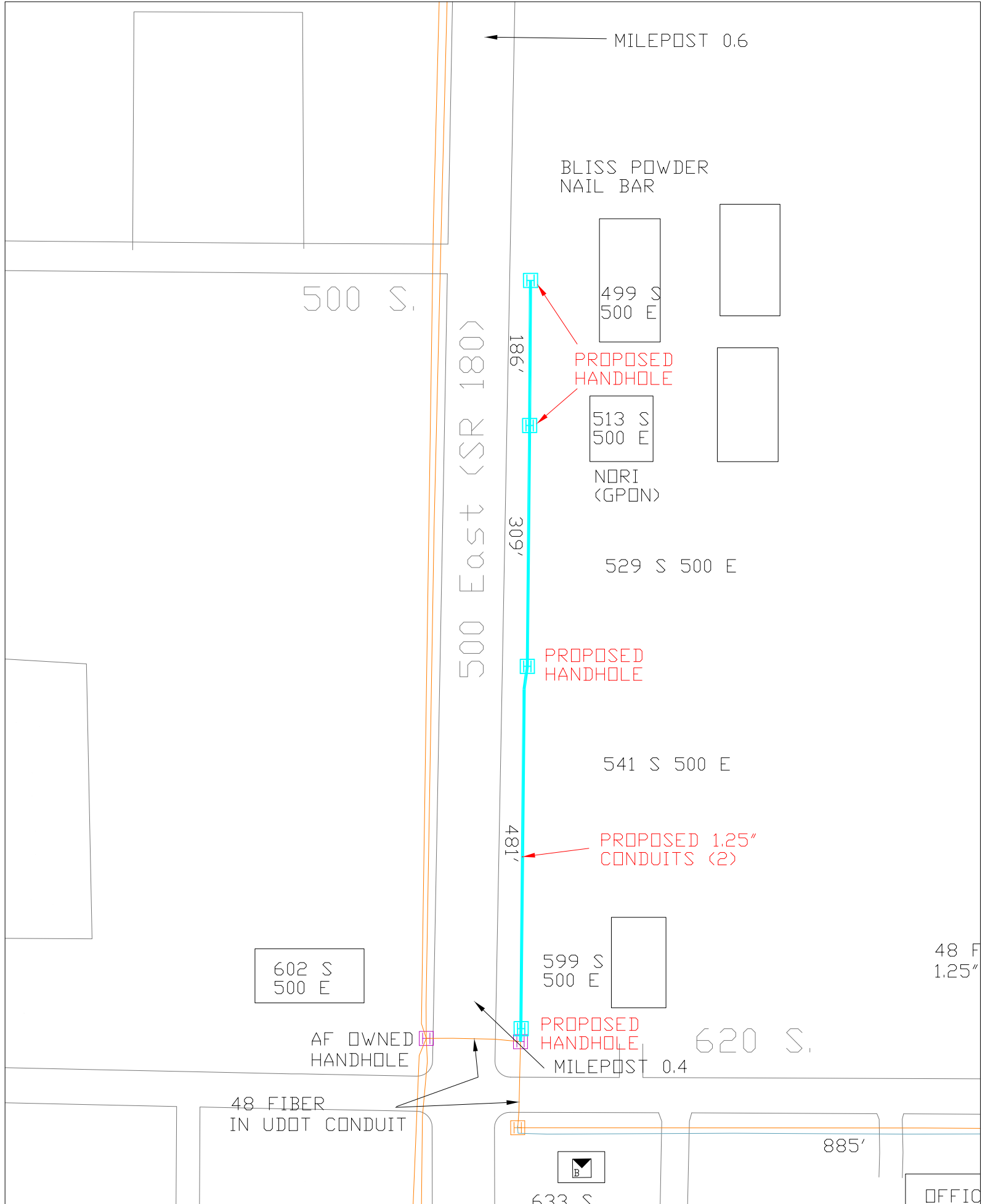
CentraCom, MC198045_MC198047: Proposed conduit path to Nori and Bliss Powder Nail Bar, 513 S and 499 S 500 East (Mileposts 0.4 to 0.6 SR 180), American Fork City, UT.
