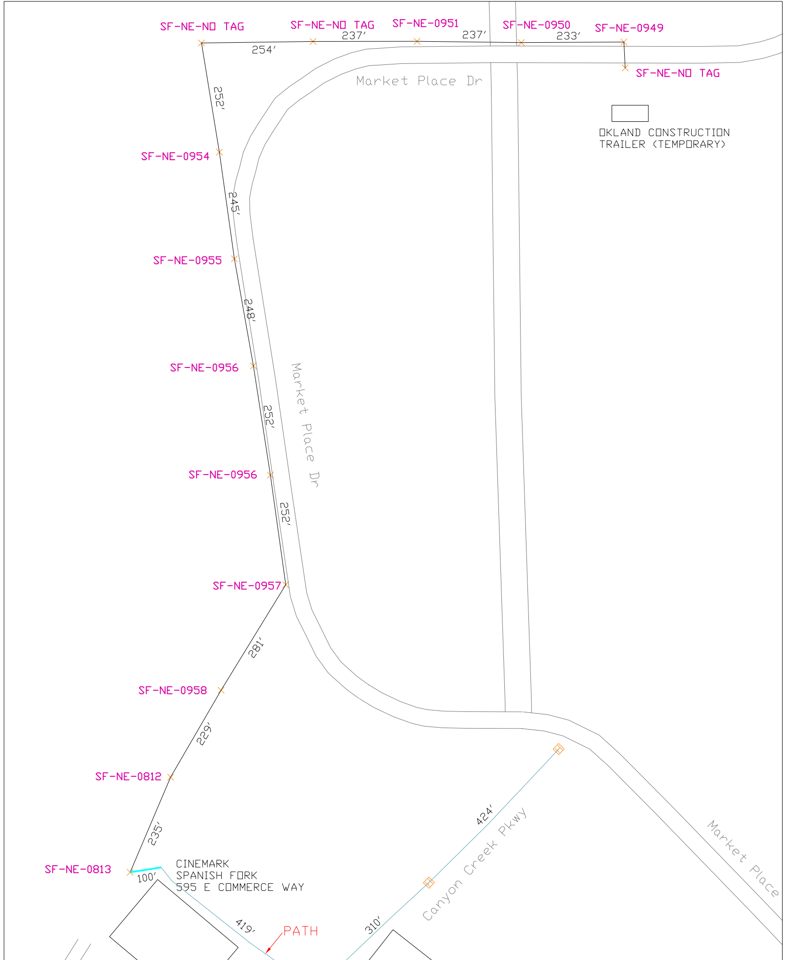
CentraCom, MC188098: Proposed location and number label of proposed Spanish Fork City poles for attachment, Market Place Drive, Spanish Fork, UT.
