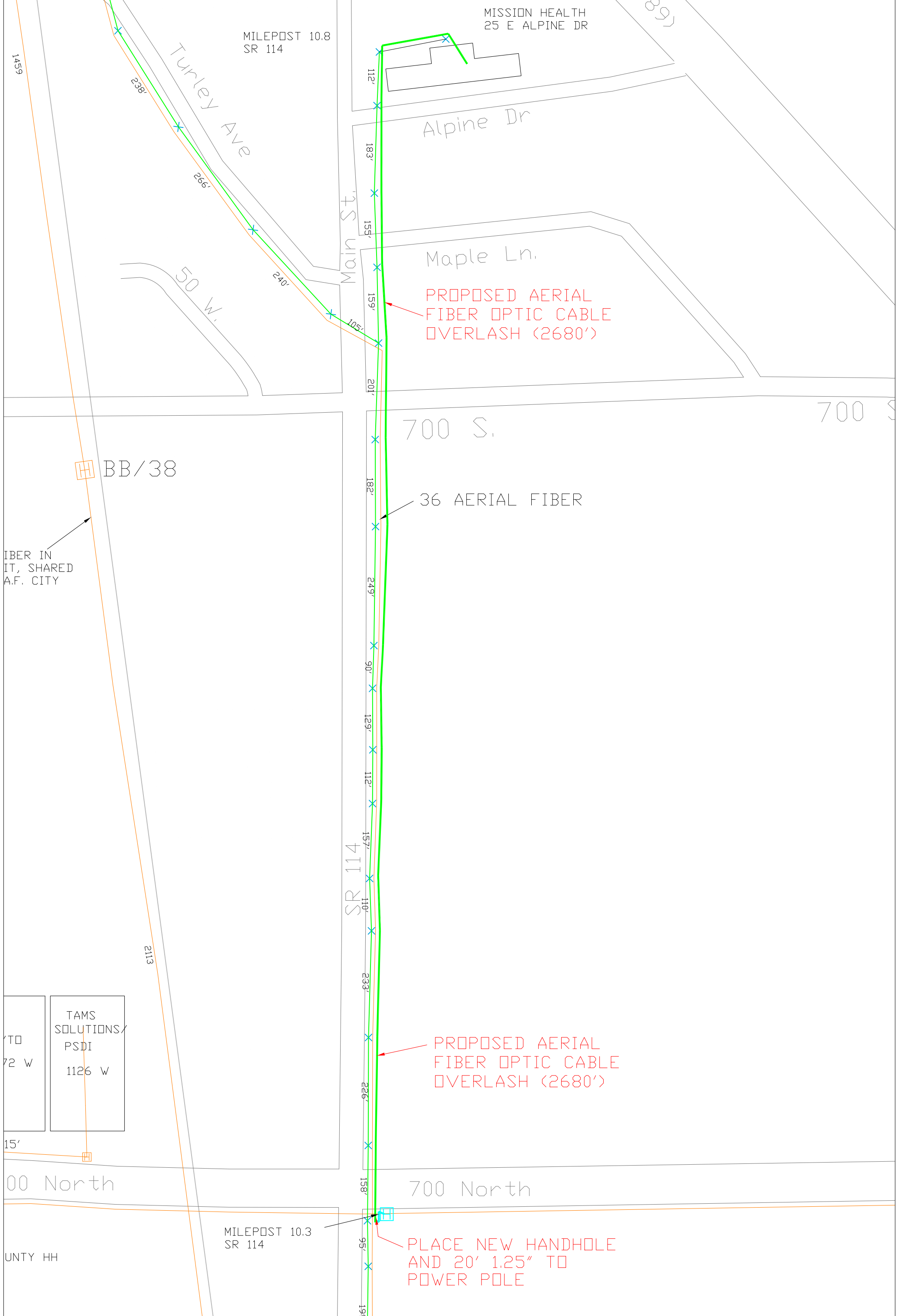
CentraCom, MC188081: Proposed fiber optic cable path to Mission Health, 25 E Alpine Dr., Pleasant Grove, UT.
