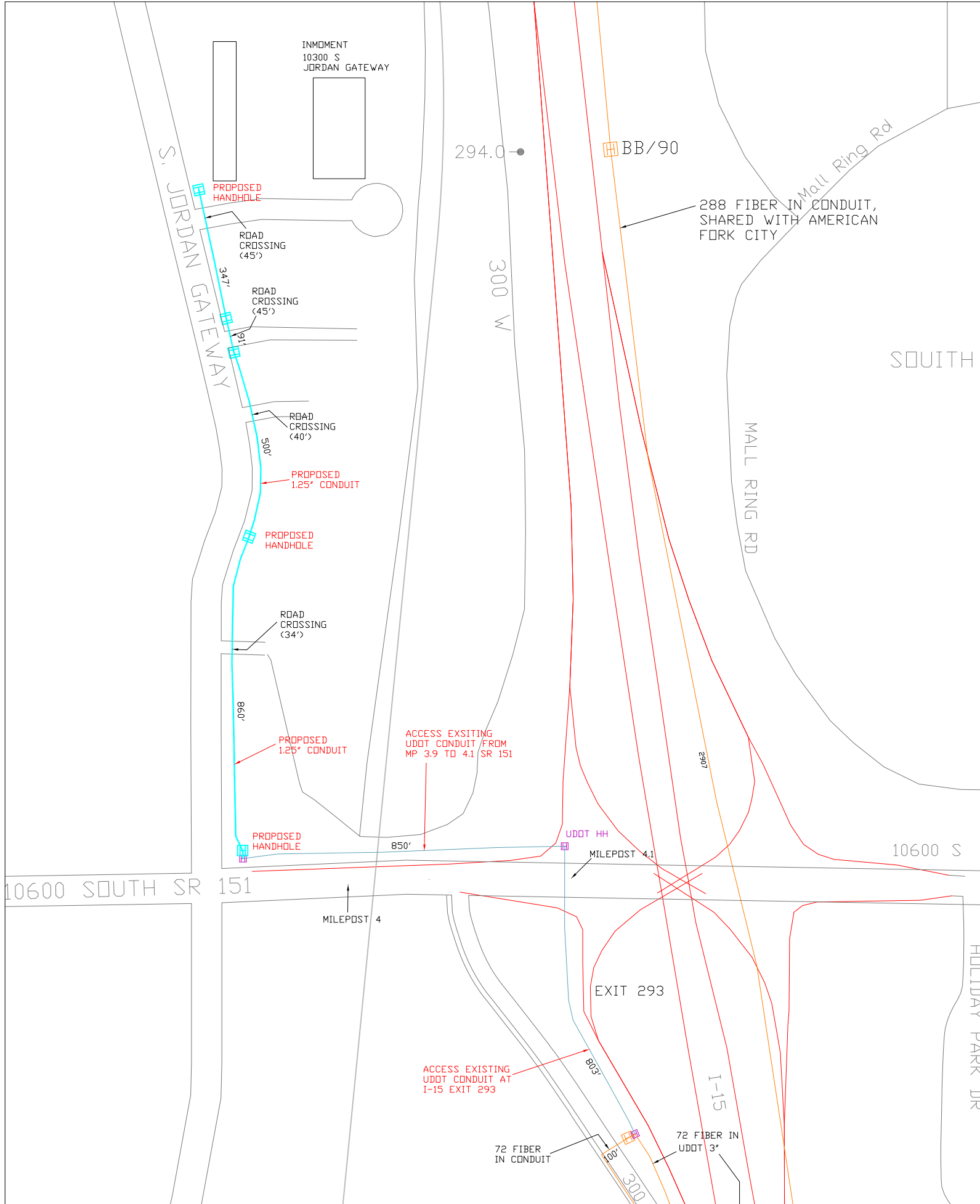
CentraCom, MC17892: Proposed conduit path to InMoment, 10300 S Jordan Gateway, South Jordan, UT.
