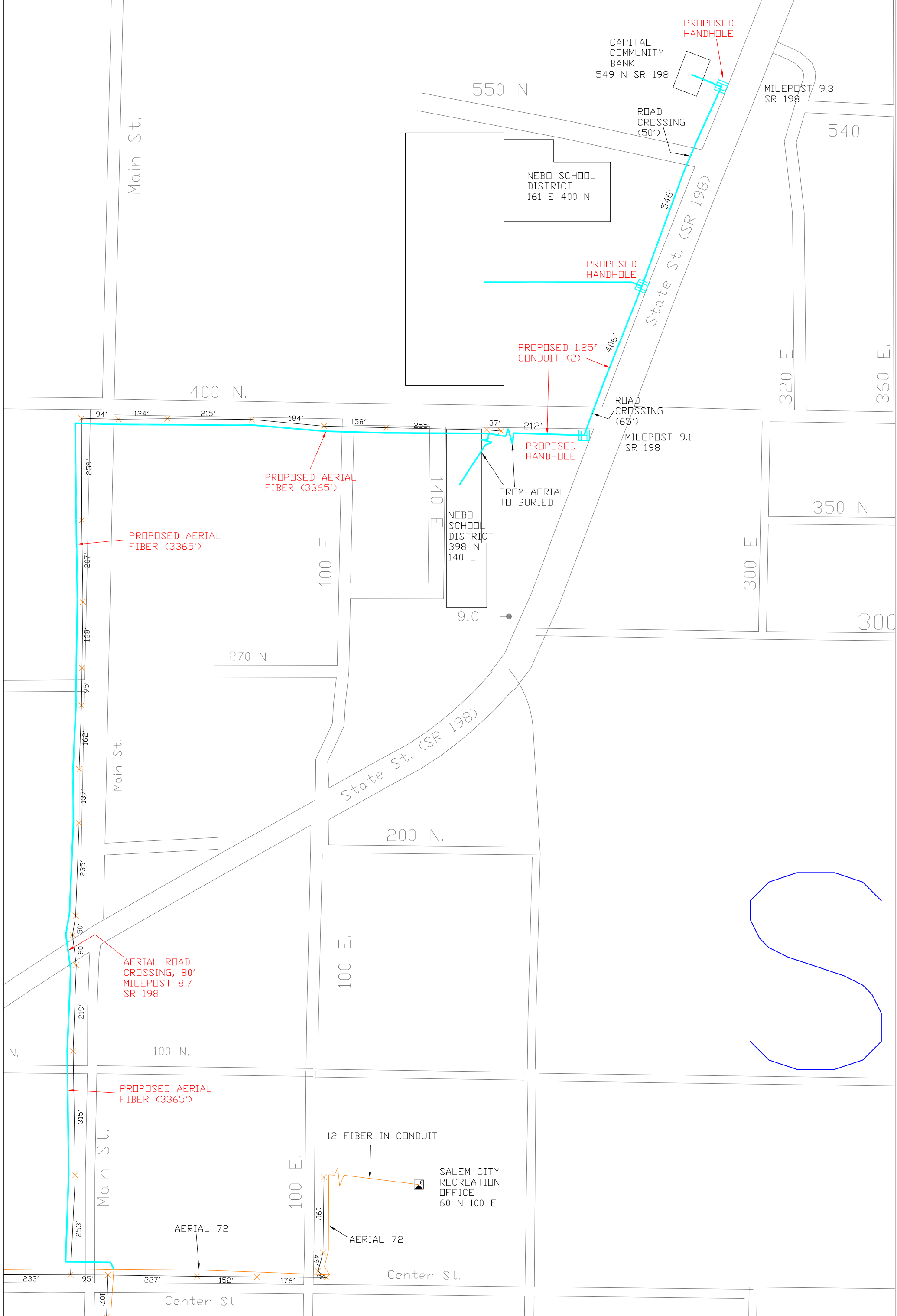
CentraCom, MC17869: Proposed fiber optic cable path to Capital Community Bank, 549 N SR 198, Salem, Ut. Also path to Nebo School District Buildings, 398 N 140 E and 161 E 400 N. Aerial crossing of SR 198 at milepost 8.7, conduit placement along SR 198 from milepost 9.1 to 9.3.
