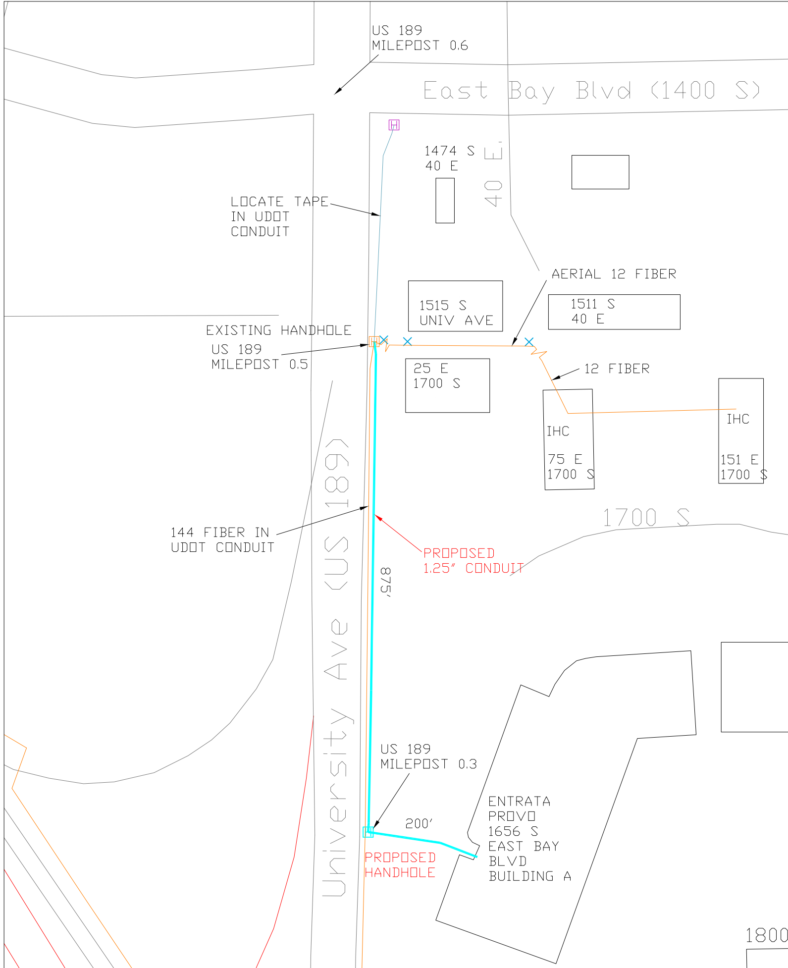
CentraCom, MC17814: Proposed conduit path to Entrata, 1656 S East Bay Blvd, Building A, Provo, UT. Taking same path as other communications provider.
