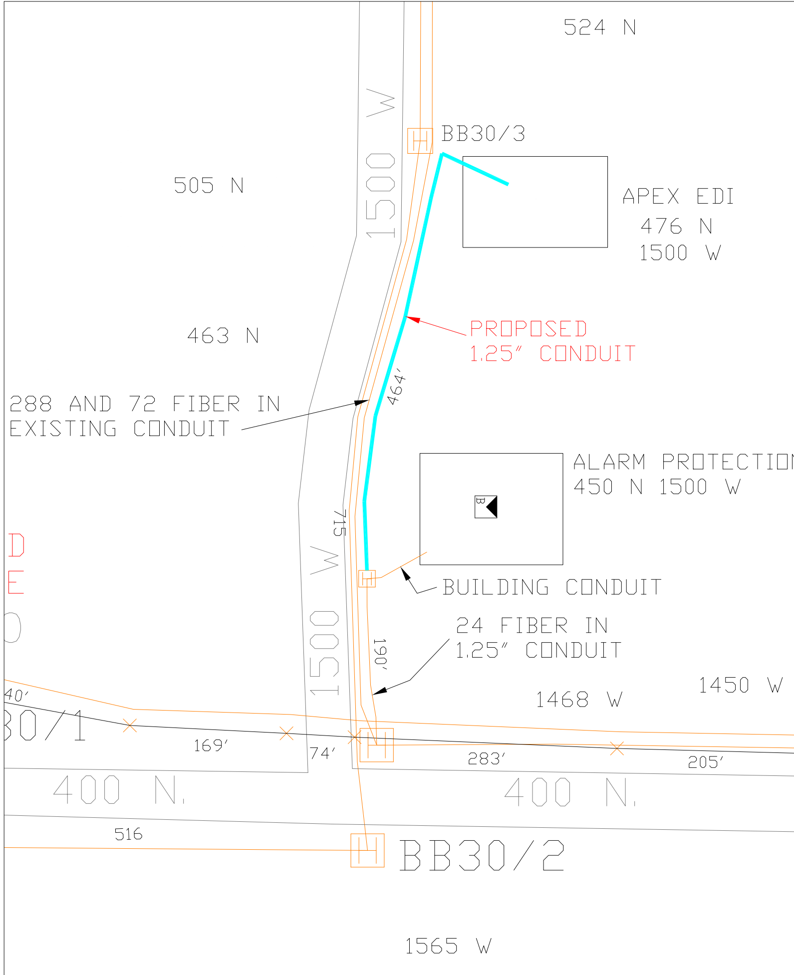
CentraCom, MC16894: Proposed conduit path to Apex EDI, 476 N 1500 W, Orem, UT.
