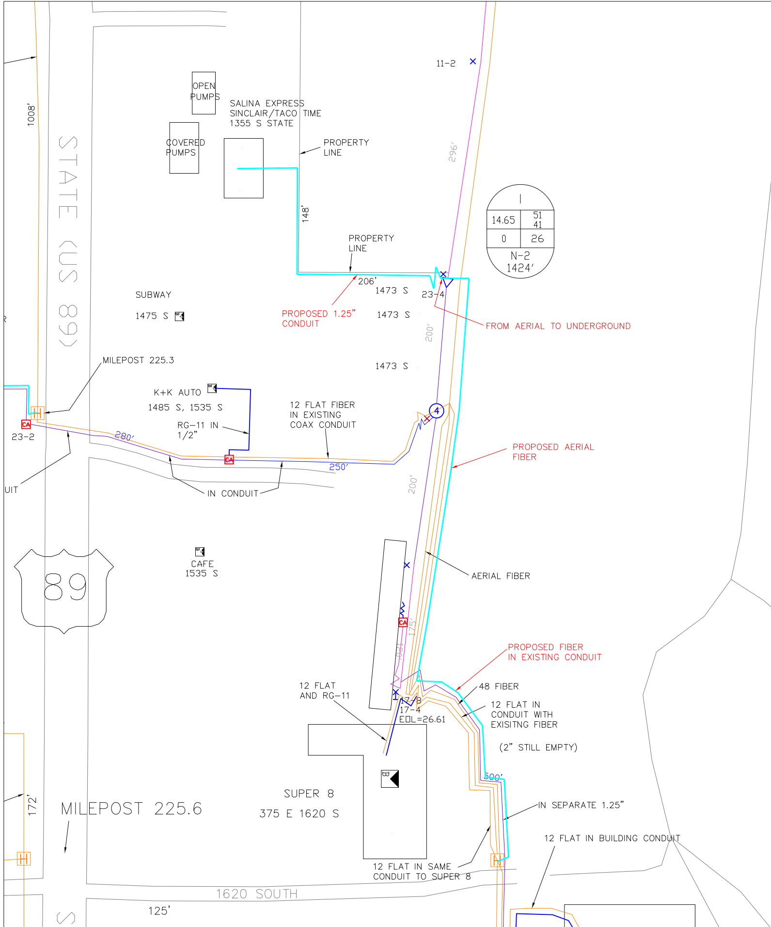
CentraCom, MC16893: Proposed conduit and fiber path to Salina Express, 1355 S State, Salina, UT.
