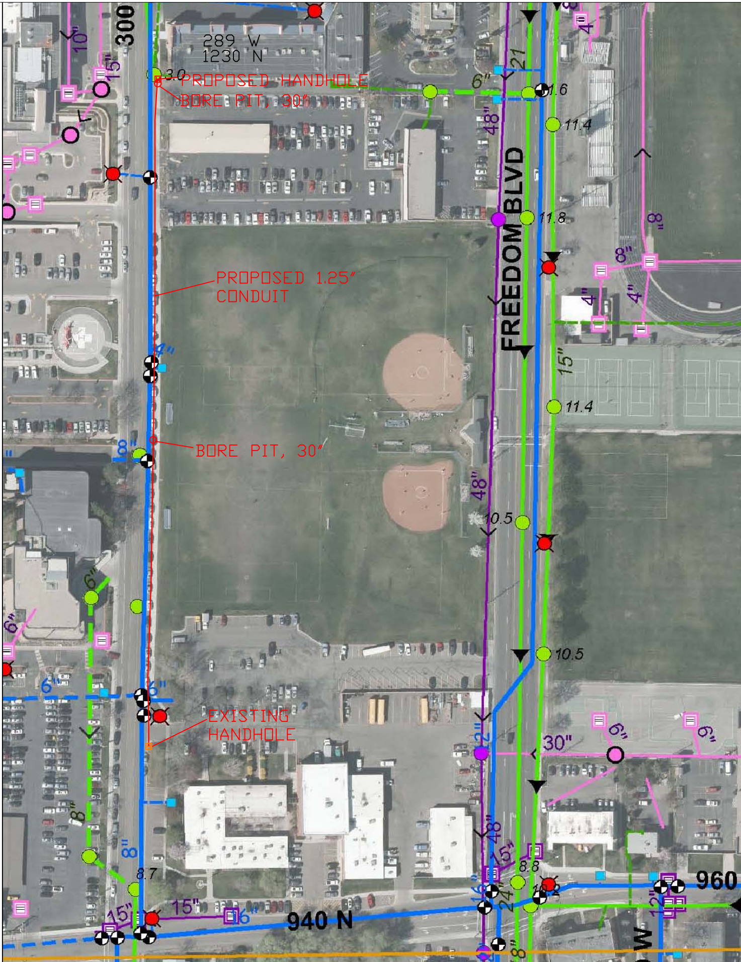
CentraCom, MC16874: Proposed conduit path to IHC Hospice 289 W 1230 N, Provo, UT. Conduit will be placed 2' back of walk at a depth of 30" avoiding existing utilities. 2 bore pits at 30" depth as shown.
