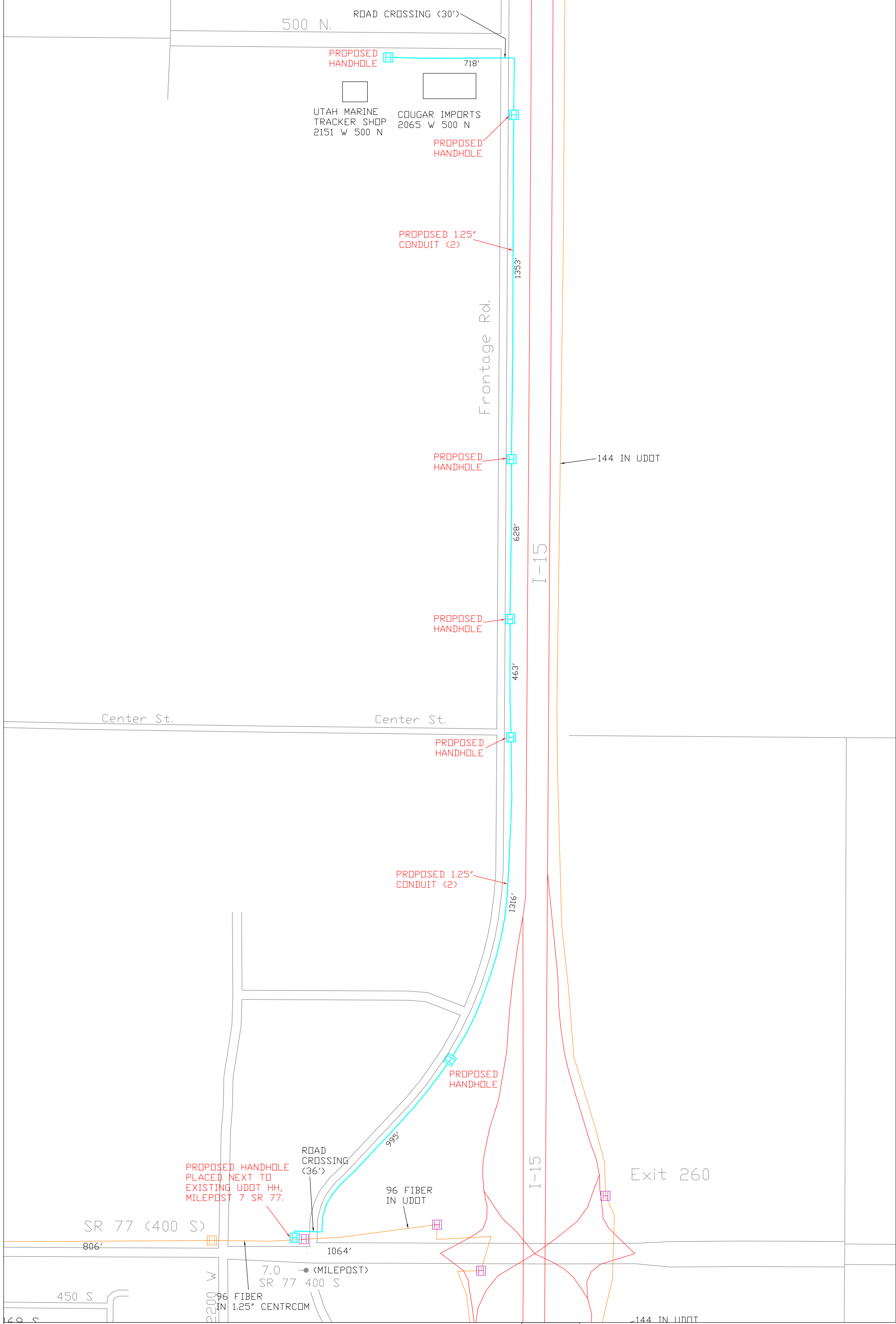
CentraCom, MC16851, Updated: Proposed conduit path to Cougar Imports and Utah Marine Tracker Shop, 2065 W 500 N and 2151 W 500 N, Springville, UT.
