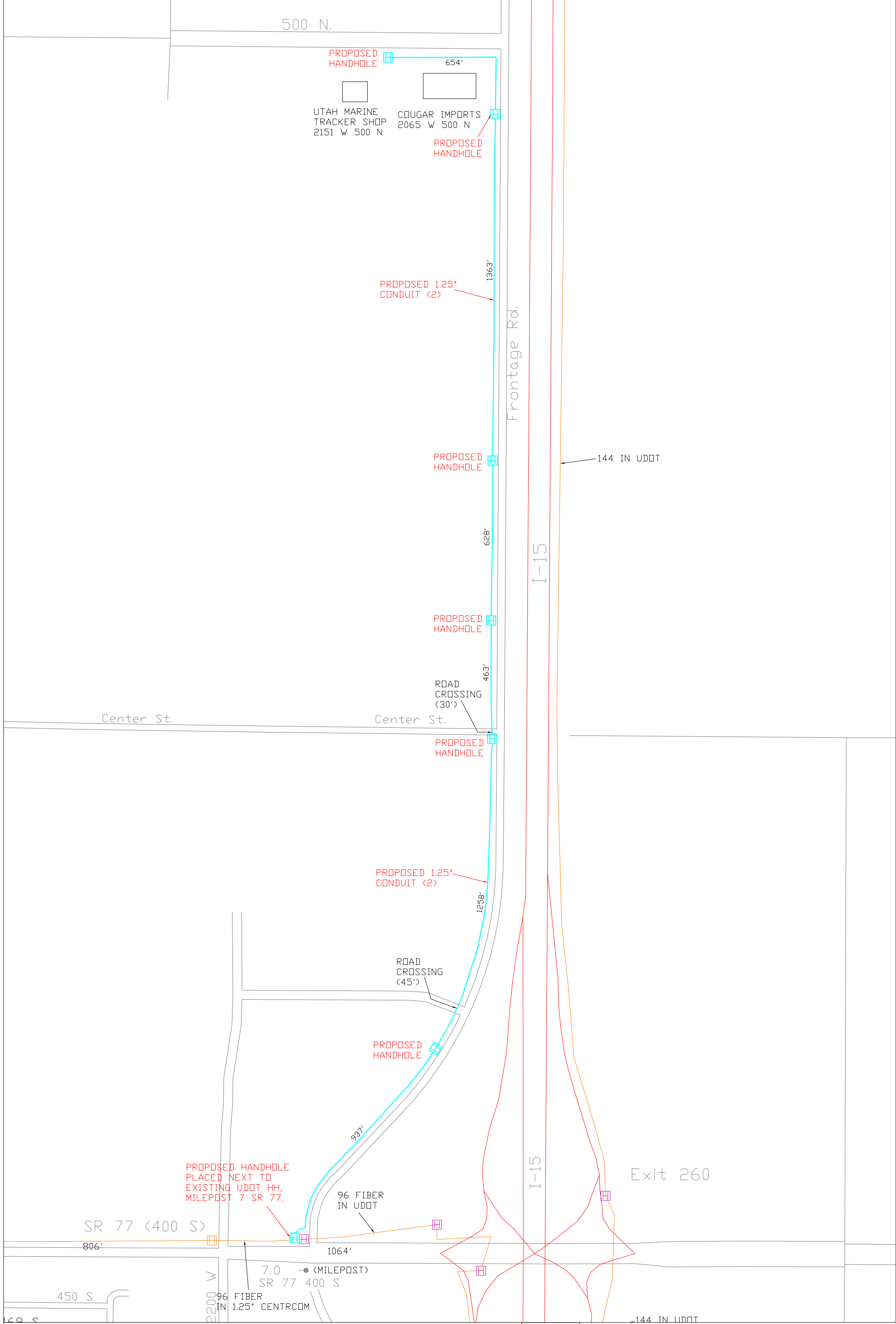
CentraCom, MC16851: Proposed conduit path to Cougar Imports and Utah Marine Tracker Shop, 2065 W 500 N and 2151 W 500 N, Springville, UT.
